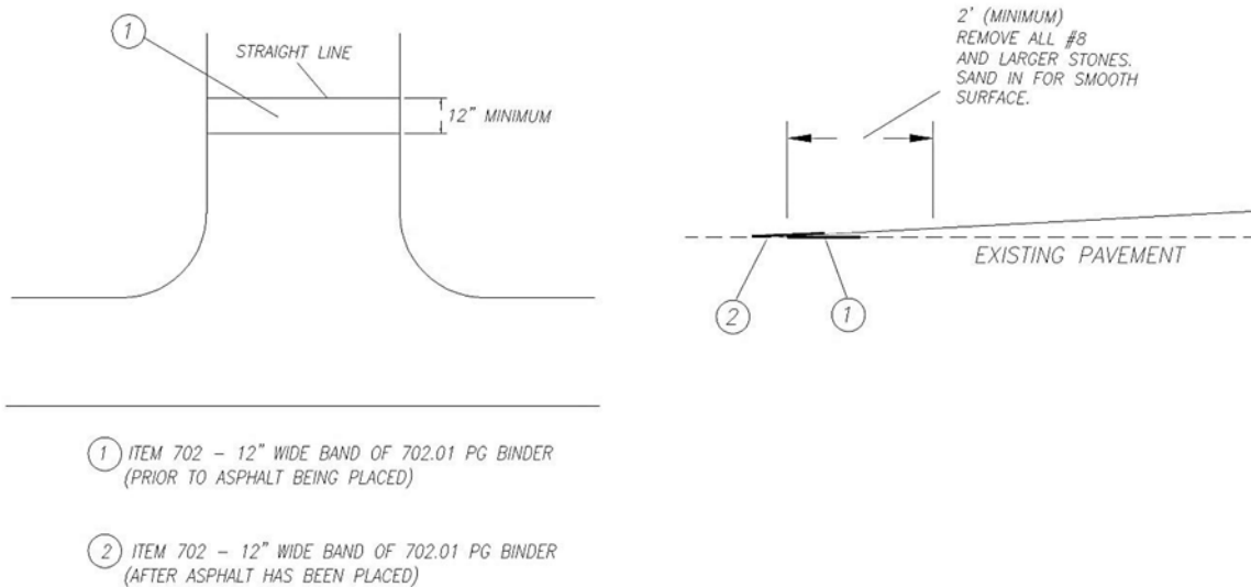
FEATHER JOINT DETAIL NO SCALE
